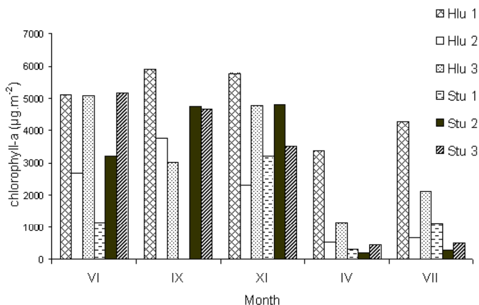
Fig. 4.2 Chlorophyll-a concentration on profiles Hluboký potok and Stuzická rieka (June 1999 – July 2000).
