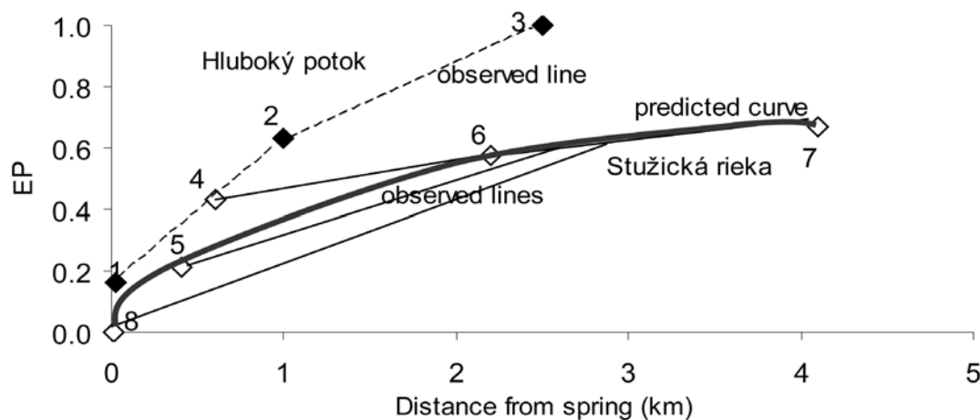
Fig. 9.3 Correspondence analysis (CA) of 8 sampling sites: 1-3 sites of the Hluboký potok, break line connected these stretch of stream; 4-8 - sites of the Stučická rieka stream basin (numbers indicate samplig sites according to explanations within Fig. 9.1), solid line connected stream stretches according to river network; EP - ecological position of sites on 1. axis (CA)
