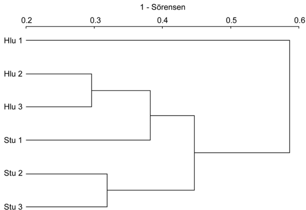
Fig. 12.1 Complete linkage dendrogram of sampling sites based on the community composition (presence/absence). Axis represents magnitude of dissimilarity (1 – Sørensen index).
