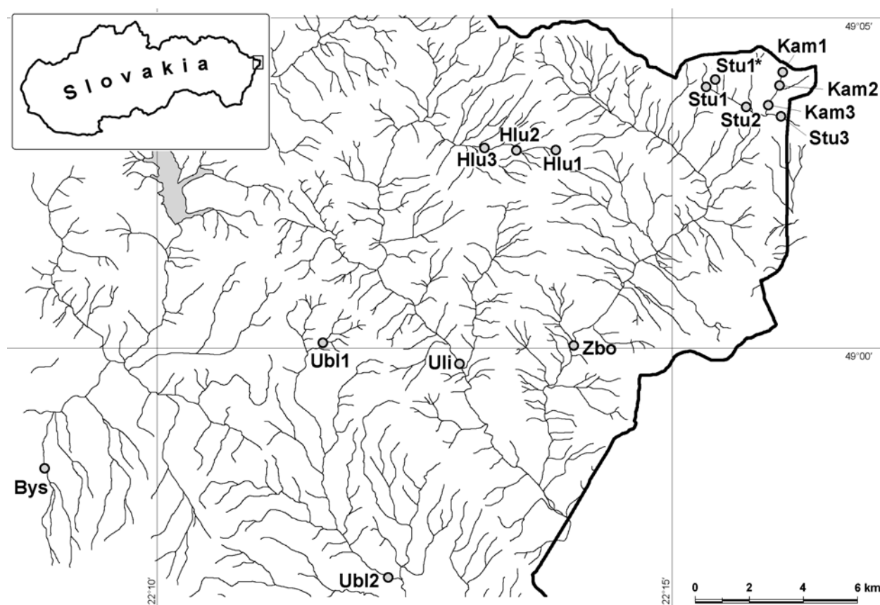
Fig. 2.1 Map of the studied area (for sampling sites codes see Tab. 1)
